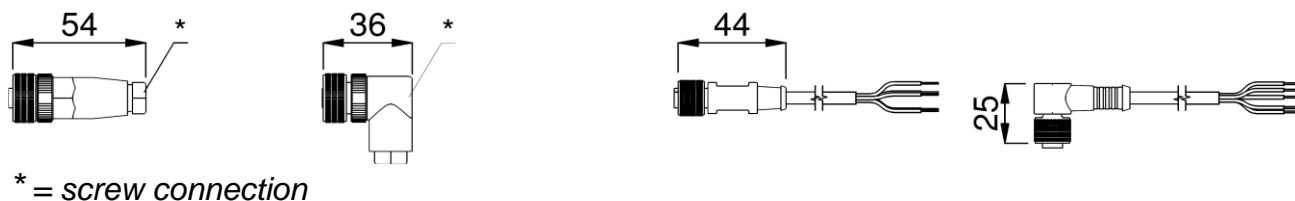
Figure 4: Optional connections
